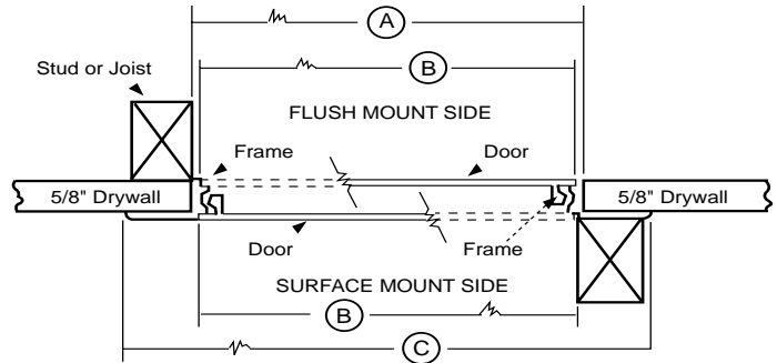
SECTION DETAIL
