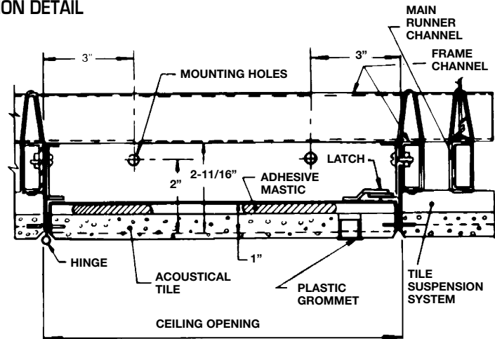
SECTION DETAIL
