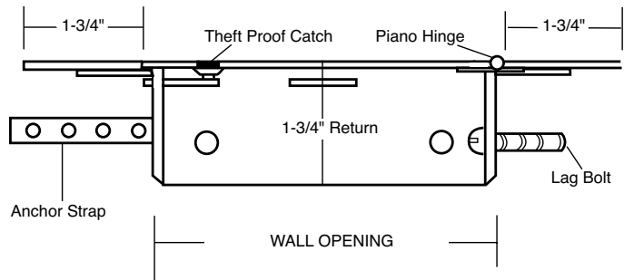
SECTION DETAIL
