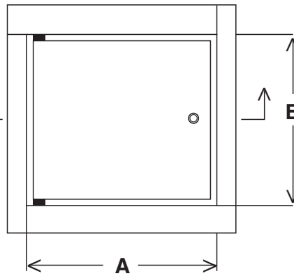
Masonry anchor straps standard on all fire-rated doors
