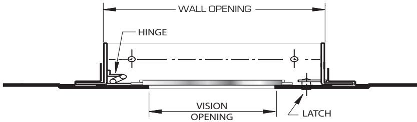
SECTION DETAIL
