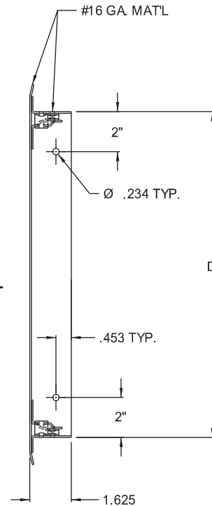
SECTION DETAIL
