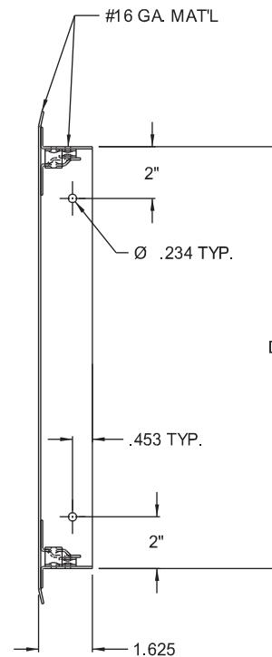
SECTION DETAIL
