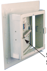
Self latching Slam Catch
