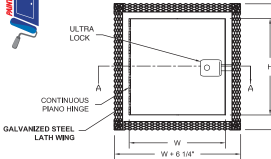
SECTION DETAIL
