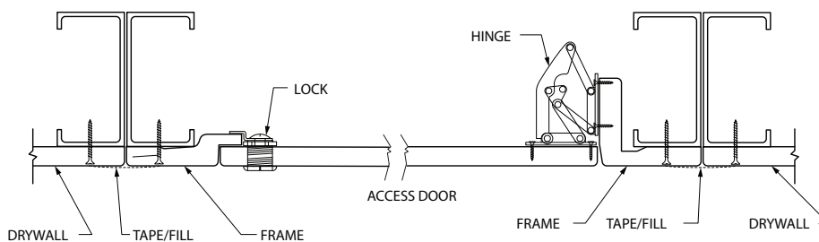
SECTION DETAIL
